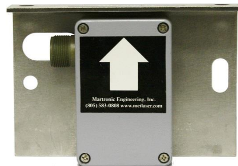
Laser-Tech Grade Control Slope Sensor
